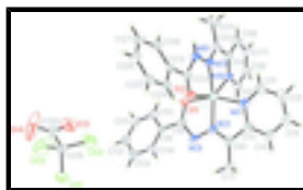
Fig. 1. The molecular structure of the title complex, showing 30% displacement ellipsoids.
